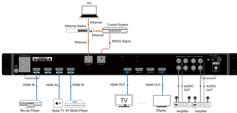
Application Diagram
