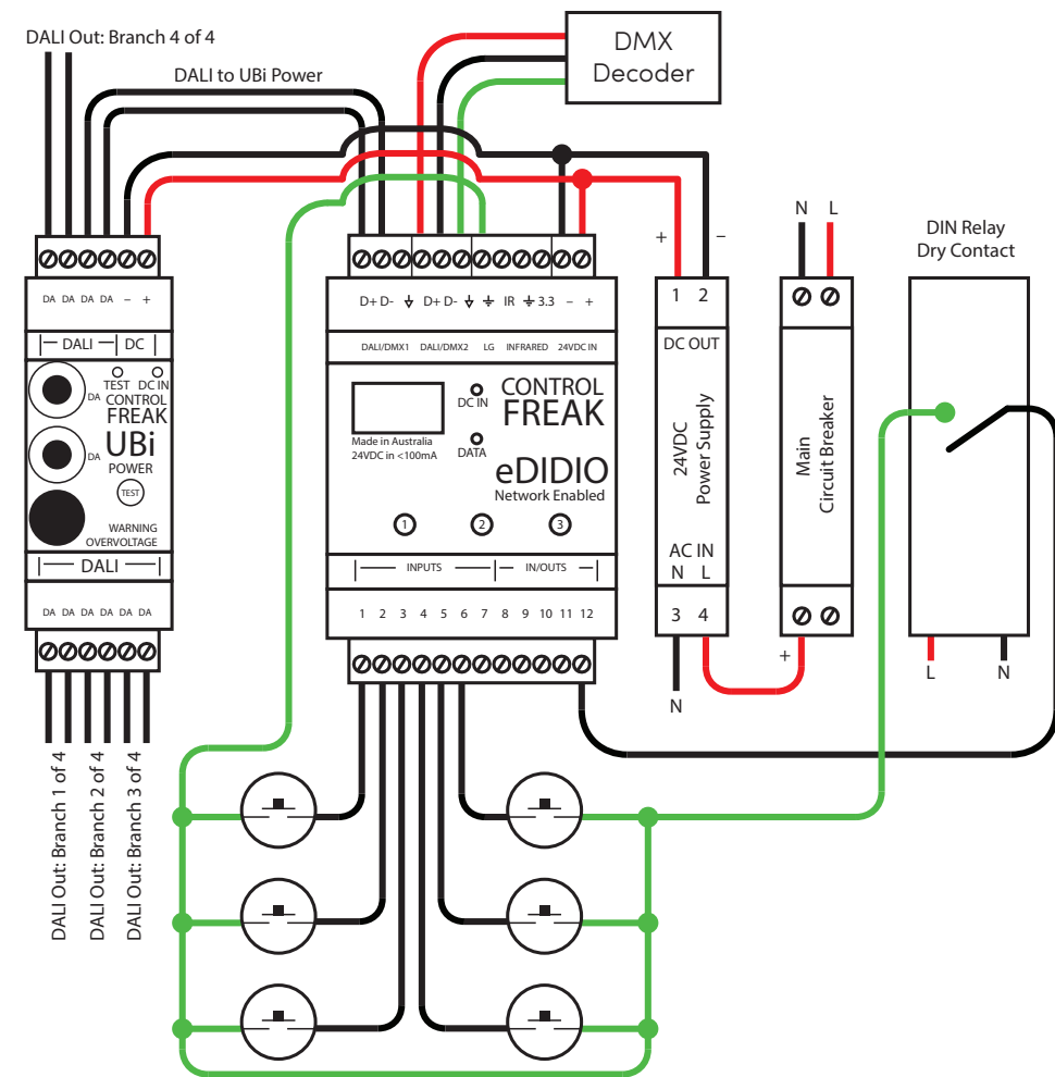
DMX decoder, DALI, and contact input connections (model CRE-EDIDIO-10-1D-1X shown)
