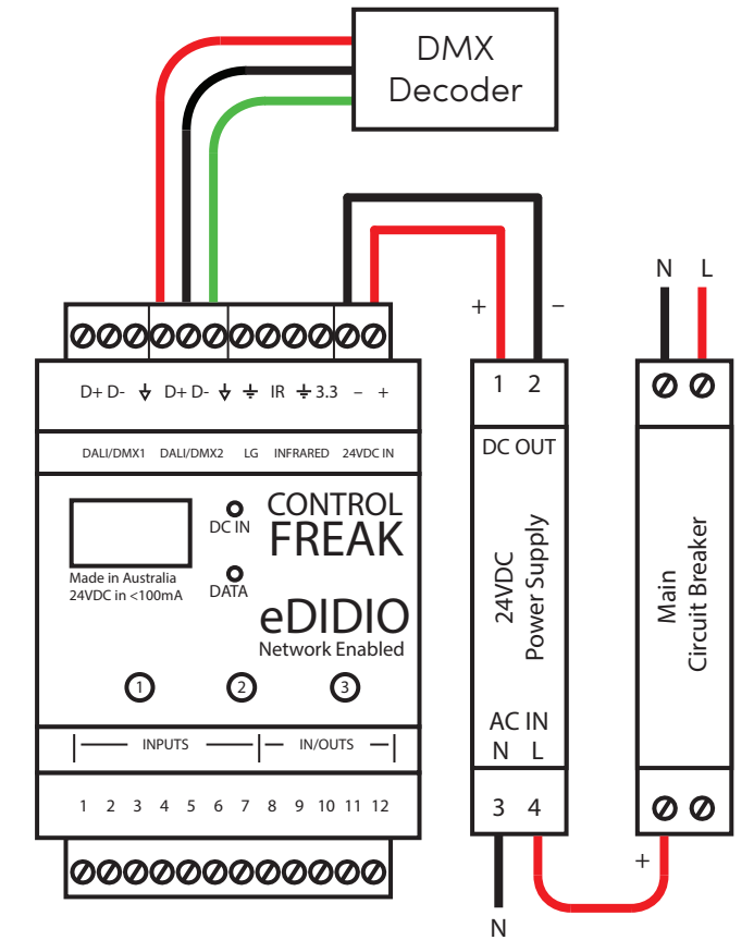
DMX decoder connections (model CRE-EDIDIO-10-1D-1X shown)
