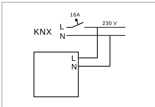
Fig. 17: Connection of network coupler
