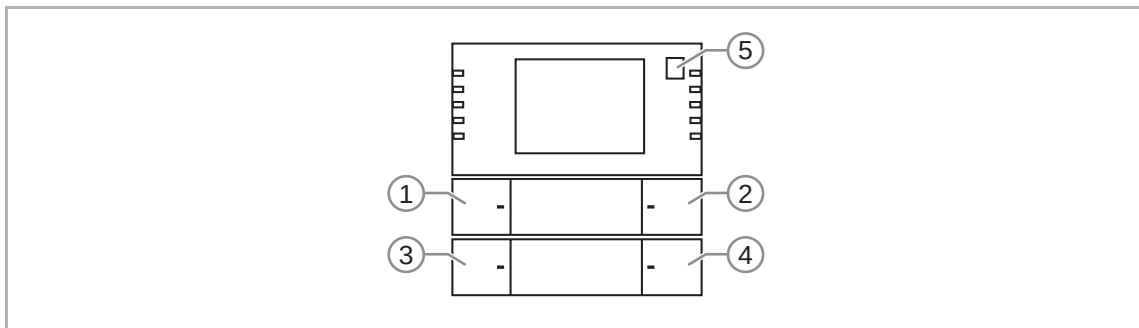
Fig. 22: RTC adjustment level: Rocker switch function
