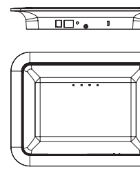
WX-1-C 802.11ac 3x3 Access Point, Plenum Rated, In-Ceiling 295 × 225 × 47 mm (11.62 × 8.87 × 1.85")
