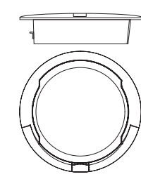
WK-2-C 802.11ac 3x3 Access Point, In-Ceiling 261 × 76 mm – radius 114 mm (10.29 × 3" – radius 4.5")
