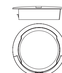
WK-1-C 802.11ac 2x2 Access Point, In-Ceiling 261 × 76 mm – radius 114 mm (10.29 × 3" – radius 4.5")
