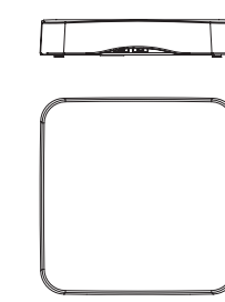
WA-4200 802.11AC 4x4 Wave 2 Access Point 207 × 207 × 37 mm (8.2 × 8.2 × 1.5")
