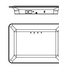
WX-1 802.11ac 3x3 Access Point, Plenum Rated 249 × 179 × 36 mm (9.80 × 7.05 × 1.43")
