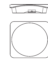
WK-1 802.11ac 2x2 Access Point 204 × 190 × 38 mm (8.02 × 7.47 × 1.49")
