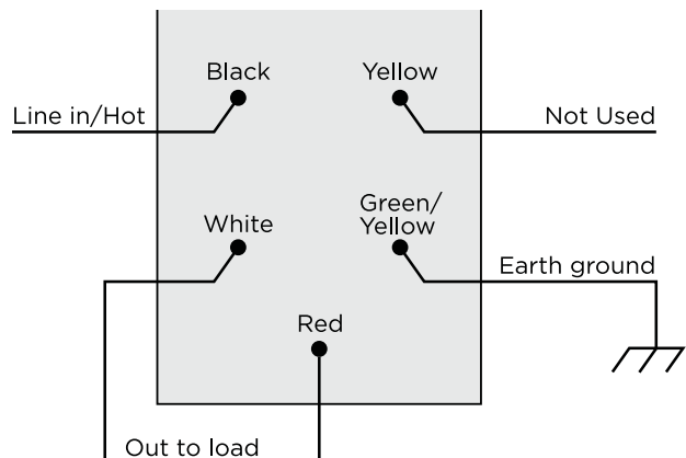
Figure 5. Single device location, without neutral connection
