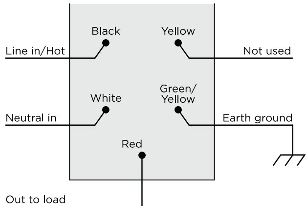
Figure 4. Single device location, with neutral connection (recommended)
