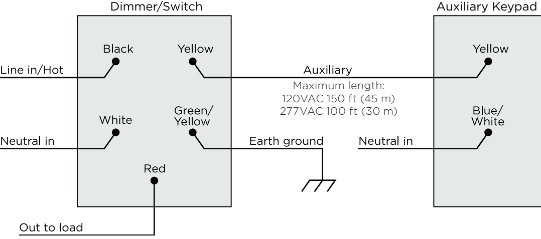
Figure 6. Multiple device location using Auxiliary Keypad, with neutral connection (recommended)
